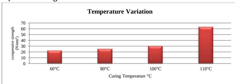
Graph No.3.7 Days Steam Curing Compressive Strength for M30
