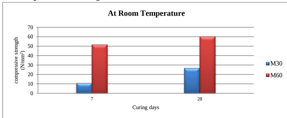
Graph No.6.7 & 28 Days Water Curing Compressive Strength for M30 &M60
